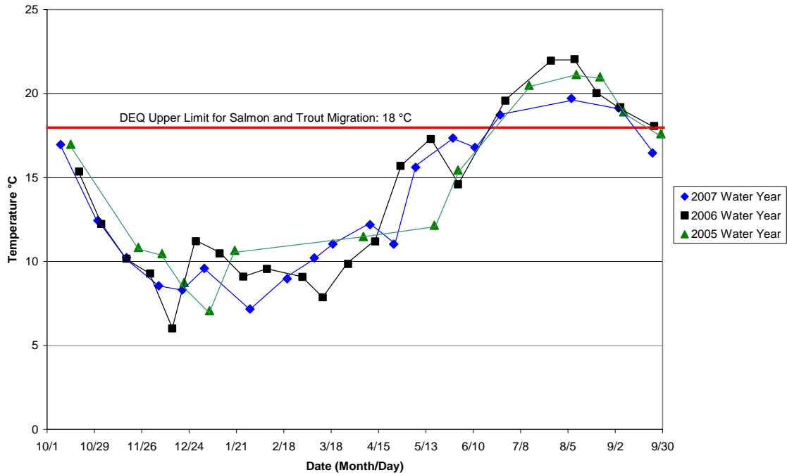
Sixes River Temperature Comparison: Water Years 2005, 2006 and 2007
