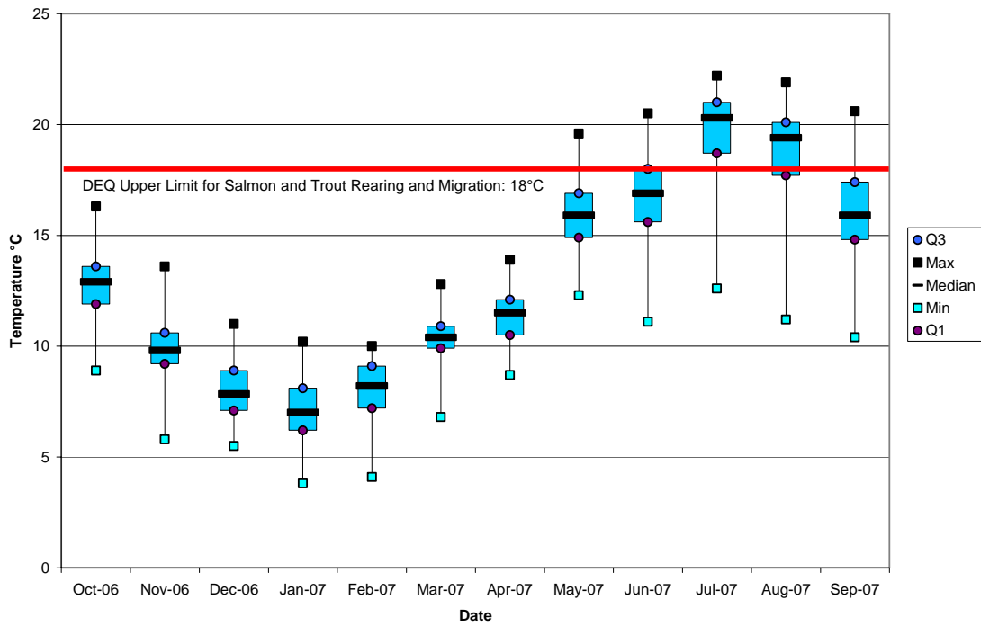
Boxplot 1.
