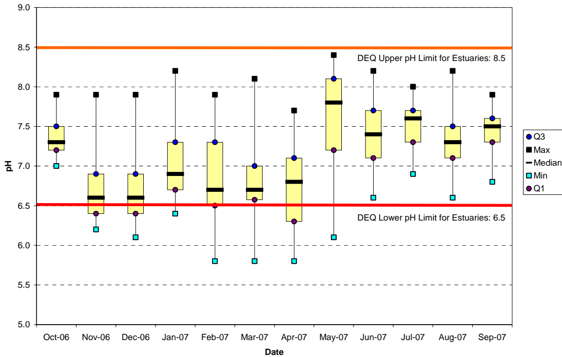
Boxplot 3.
