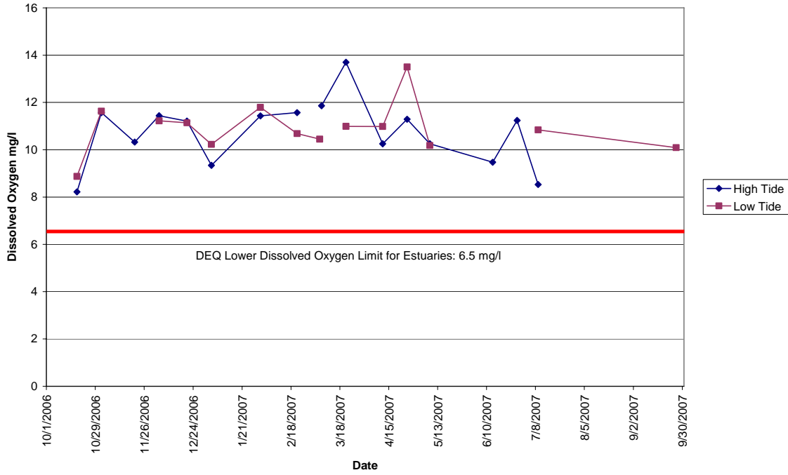
Kentuck Slough High Tide v. Low Tide Dissolved Oxygen Comparison: Water Year 2007
