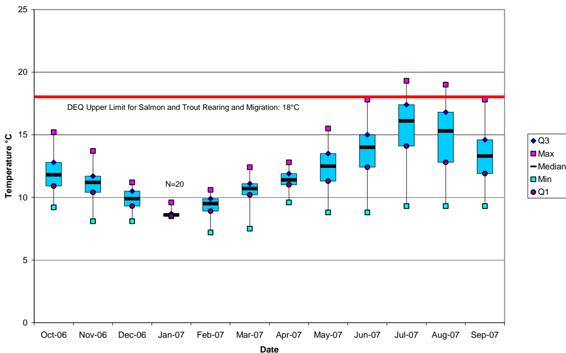
Boxplot 7
