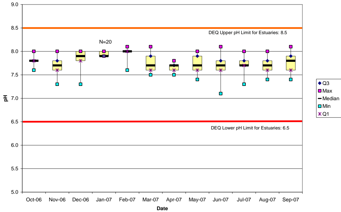
Boxplot 9
