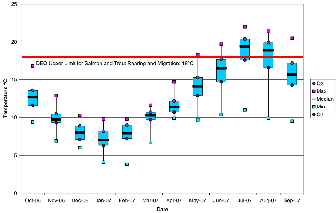
Boxplot 4
