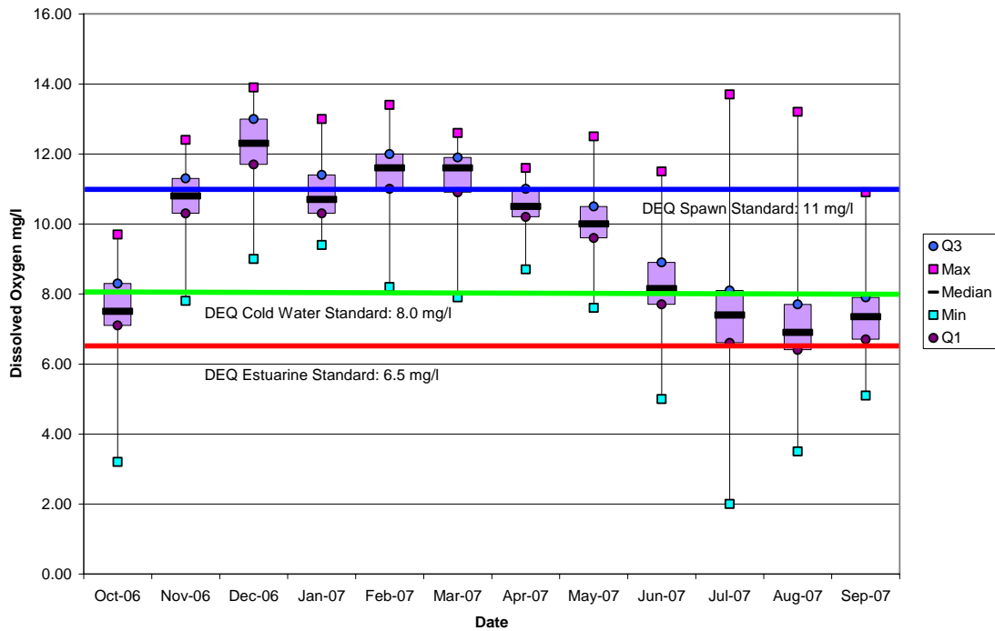
Boxplot 5
