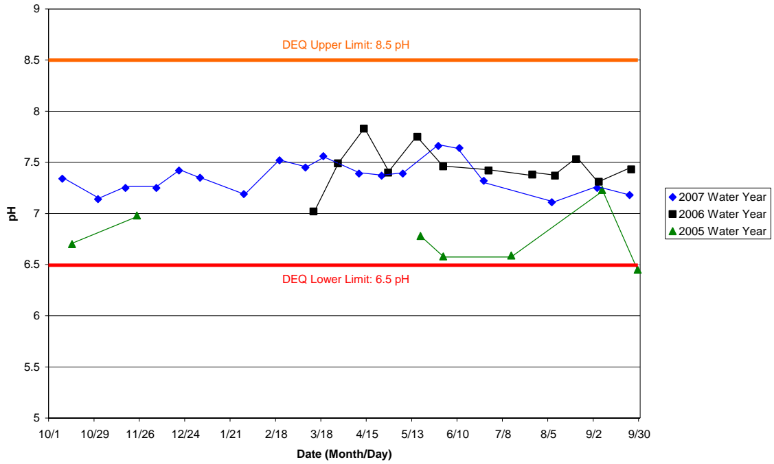
Sixes River pH Comparisons: Water Years 2005, 2006 and 2007
