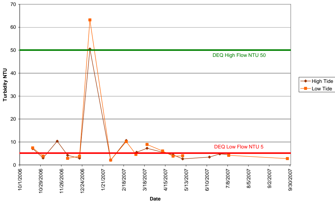
Kentuck Slough High Tide v. Low Tide Turbidity Comparison: Water Year 2007
