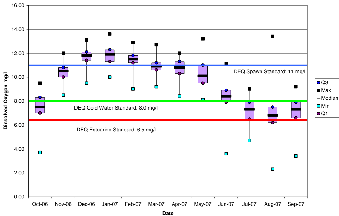
Boxplot 2.
