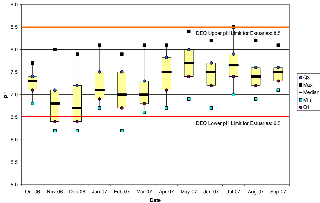
Boxplot 6
