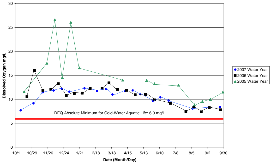
Sixes River Dissolved Oxygen Comparison: Water Years 2005, 2006 and 2007
